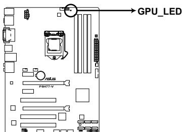
LED GPU Boost de la P8H77-V
