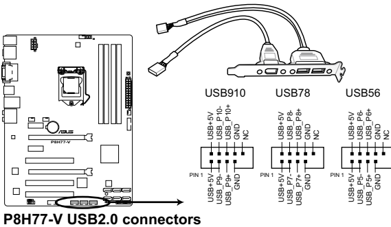
P8H77-V USB2.0 connectors
