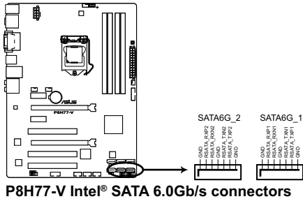
P8H77-V Intel® SATA 6.0Gb/s connectors
