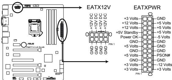
P8Z77-V LE PLUS ATX power connectors
