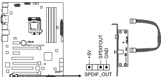
P8277-V LE PLUS Digital audio connector
