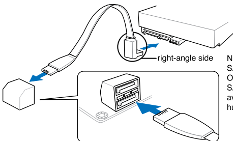
P8Z77-V LE PLUS Intel SATA 3.0Gb/s connectors
