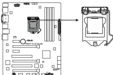
P8Z77-V LE PLUS CPU socket LGA1155
