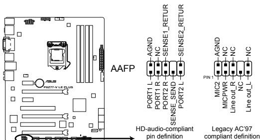
P8277-V LE PLUS Front panel audio connector
