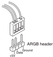
+5V Data Ground
