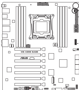
WS X299 SAGE CPU/ DRAM/ BOOT_DEVICE/ VGA LED
