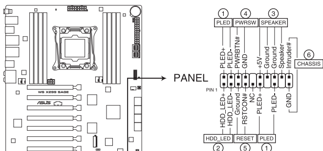
WS X299 SAGE System panel connector
