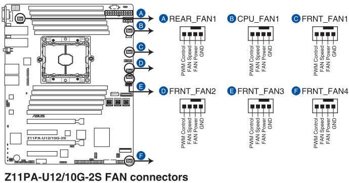
Z11PA-U12/10G-2S FAN connectors
