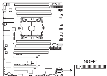
Z11PA-U12/10G-2S NGFF connector
