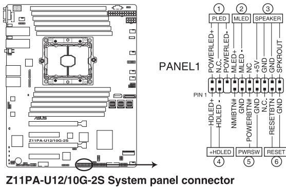
Z11PA-U12/10G-2S System panel connector
