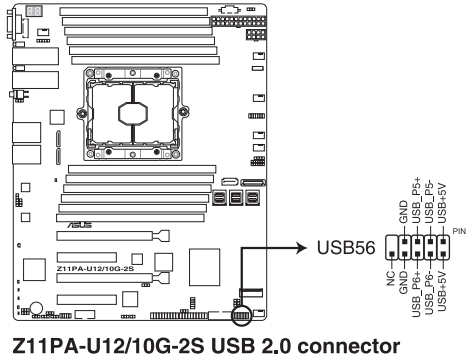
Z11PA-U12/10G-2S USB 2.0 connector
