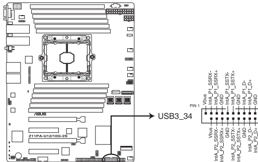
Z11PA-U12/10G-2S USB 3.0 connector
