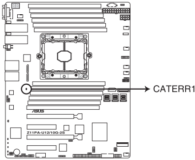
Z11PA-U12/10G-2S CATTERR LED
