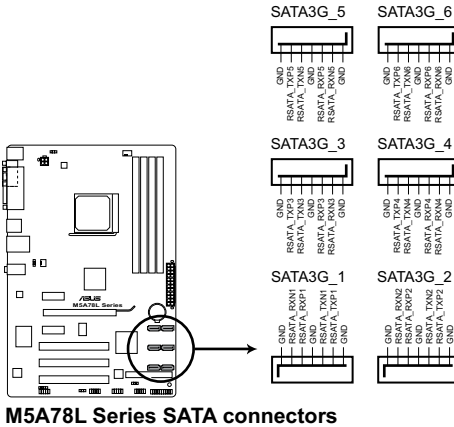
M5A78L Series SATA connectors
