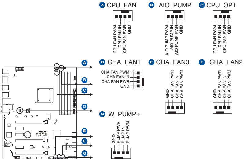
PRIME X570-PRO Fan connectors
