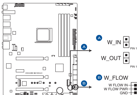
ROG CROSSHAIR VIII FORMULA Water Cooling System connectors
