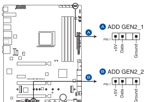
ROG CROSSHAIR VIII FORMULA Addressable RGB LED connector
