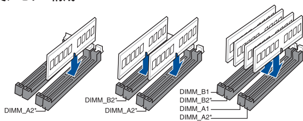
ROG CROSSHAIR VIII FORMULA 288-pin DDR4 DIMM socket
