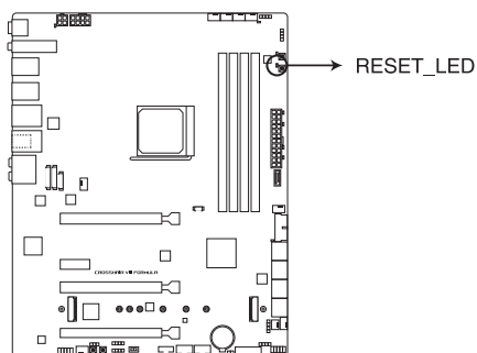
ROG CROSSHAIR VIII FORMULA RESET LED
