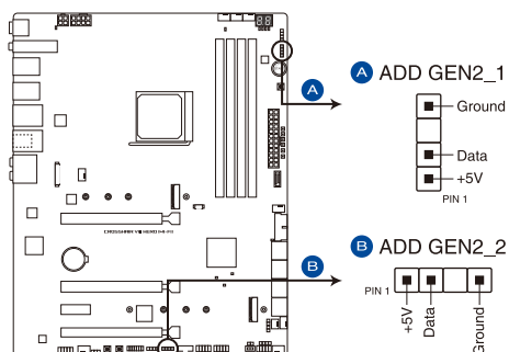
ROG CROSSHAIR VIII HERO (WI-FI) Addressable RGB LED connector
