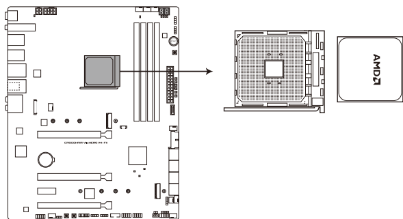
ROG CROSSHAIR VIII HERO (WI-FI) CPU AM4
