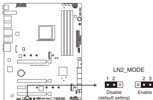
ROG CROSSHAIR VIII HERO (WI-FI) LN2 Mode jumper
