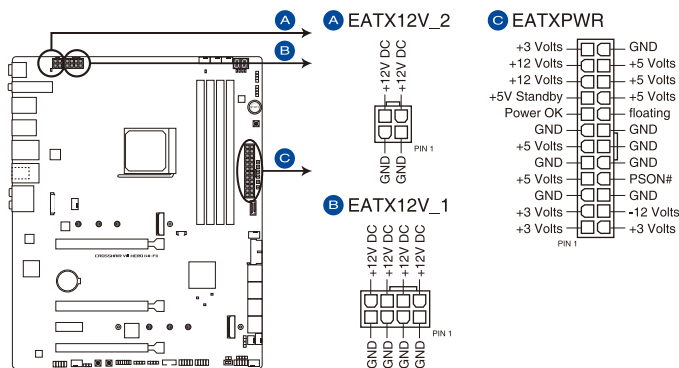
ROG CROSSHAIR VIII HERO (WI-FI) Power connectors
