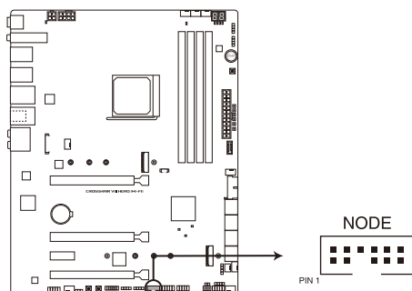
ROG CROSSHAIR VIII HERO (WI-FI) Node connector
