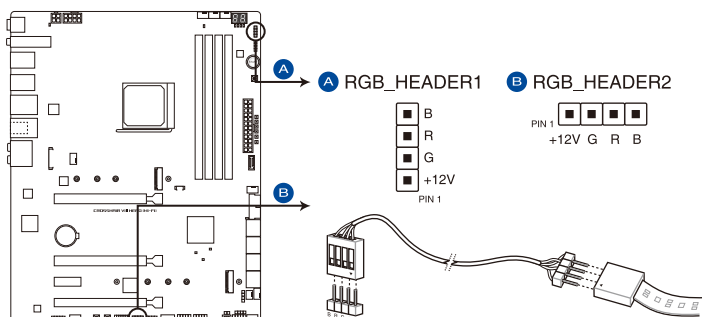
ROG CROSSHAIR VIII HERO (WI-FI) AURA RGB LED connector
