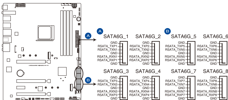
ROG CROSSHAIR VIII HERO (WI-FI) SATA 6 Gb/s connector
