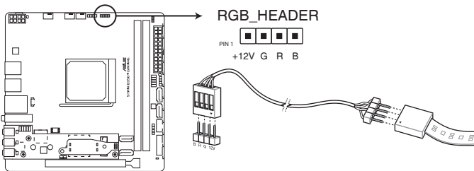
ROG STRIX B350-I GAMING RGB header
