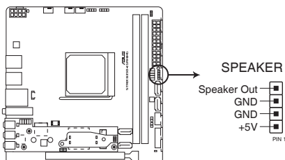
ROG STRIX B350-I GAMING Speaker out connector
