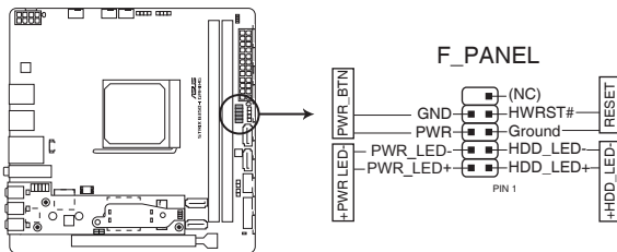
ROG STRIX B350-I GAMING System panel connector
