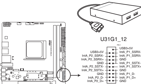
ROG STRIX B350-I GAMING USB3.1 Gen1 connector
