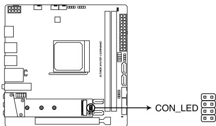
ROG STRIX X470-I GAMING CON_LED
