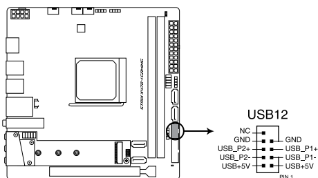
ROG STRIX X470-I GAMING USB 2.0 connector
