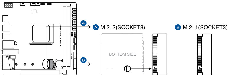
ROG STRIX X470-I GAMING M.2 socket
