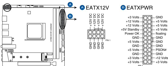
ROG STRIX X470-I GAMING ATX power connectors
