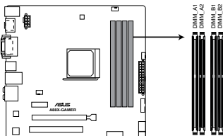
A88X-GAMER 240-pin DDR3 DIMM sockets
