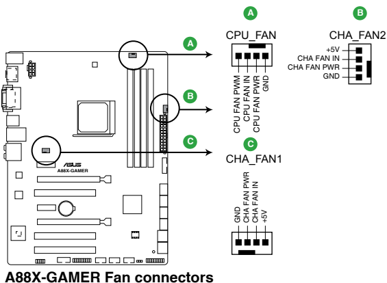
A88X-GAMER Fan connectors
