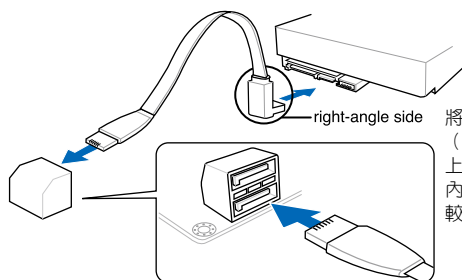
A88X-PRO SATA 6.0Gb/s connectors
