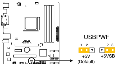
A88XM-A USB device wake up
