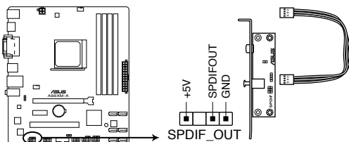
A88XM-A Digital audio connector
