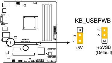
A88XM-A Keyboard and USB device wake up
