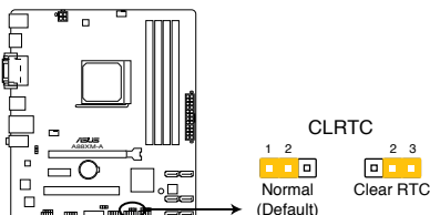
A88XM-A Clear RTC RAM
