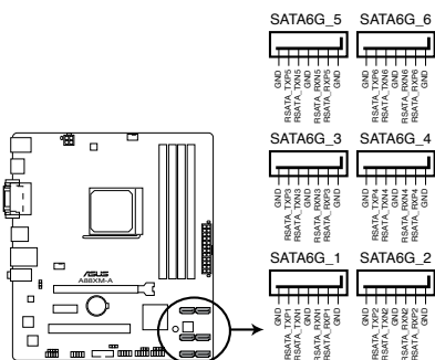
A88XM-A SATA 6.0Gb/s connectors
