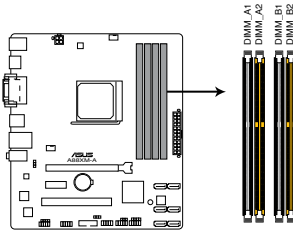
A88XM-A 240-pin DDR3 DIMM sockets
