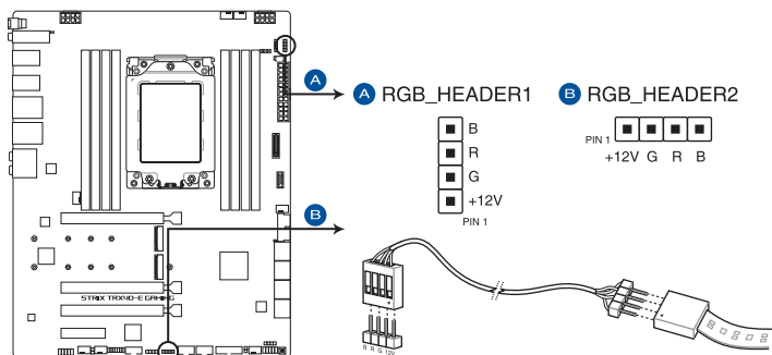
ROG STRIX TRX40-E GAMING AURA RGB LED connector
