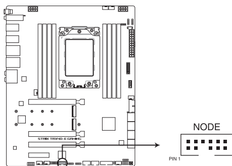
ROG STRIX TRX40-E GAMING Node connector
