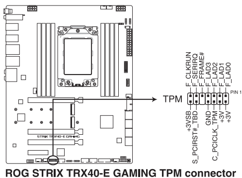
ROG STRIX TRX40-E GAMING TPM connector
