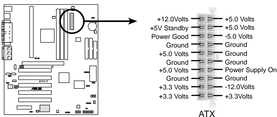
K7V-T ATX Power Connector
