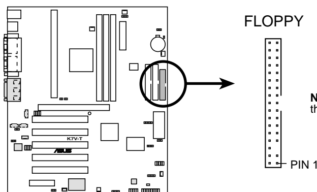
K7V-T Floppy Disk Drive Connector
