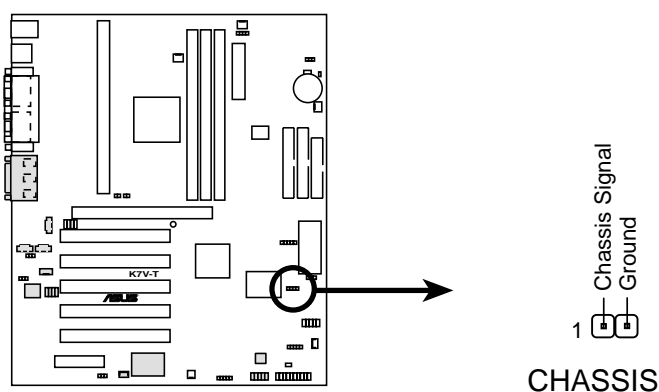
K7V-T Chassis Open Alarm Lead
