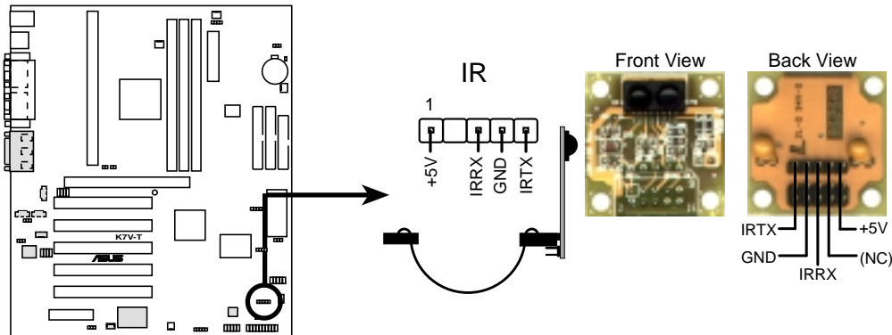
K7V-T Infrared Module Connector
