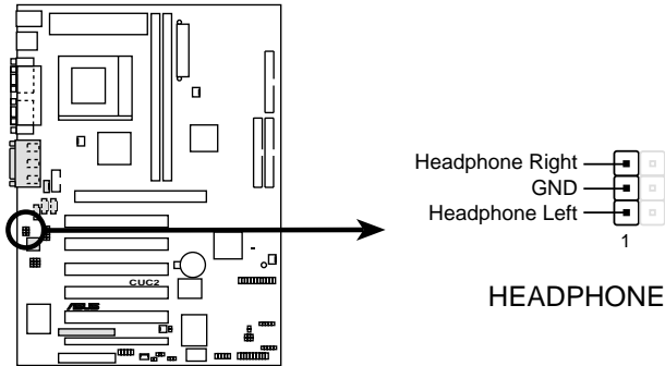
CUC2 True-Level Line Out Header
