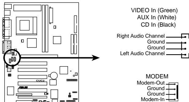
CUC2 Internal Audio Connectors
