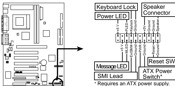
CUC2 System Panel Connectors
