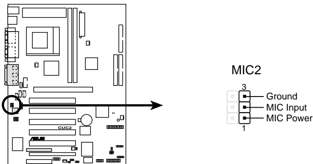
CUC2 Internal Microphone Connector
