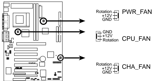
CUC2 12-Volt Cooling Fan Power
