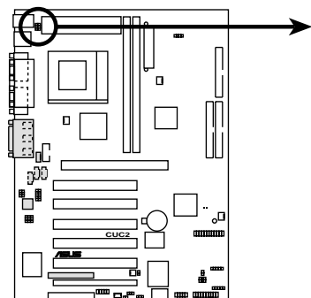
CUC2 Keyboard Power Setting
