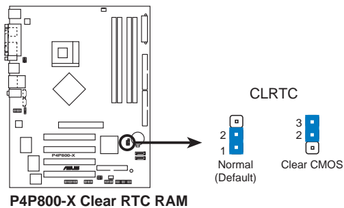
P4P800-X Clear RTC RAM
