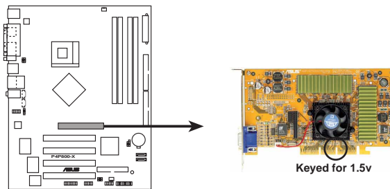
P4P800-X Accelerated Graphics Port (AGP)
