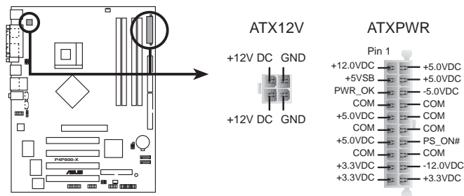
P4P800-X ATX power connectors
