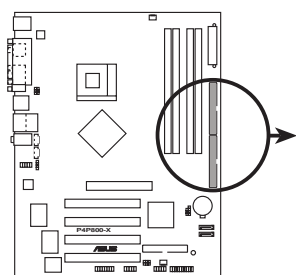
P4P800-X IDE connectors
