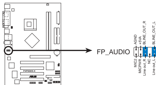
P4P800S-X Front Panel Audio Connector
