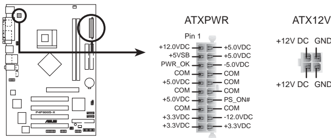
P4P800S-X ATX Power Connectors
