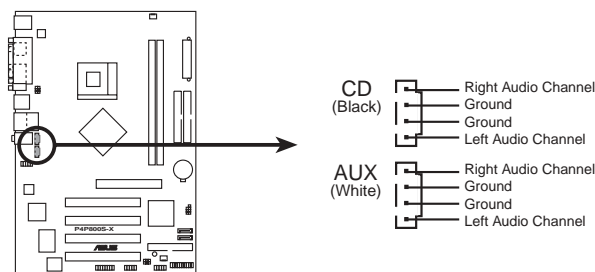
P4P800S-X Internal Audio Connectors
