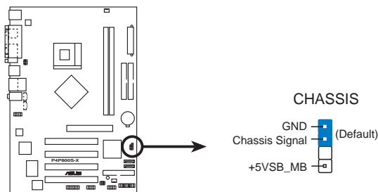
P4P800S-X Chassis Alarm Lead
