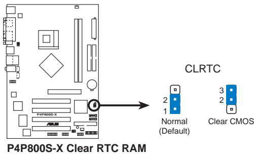
P4P800S-X Clear RTC RAM
