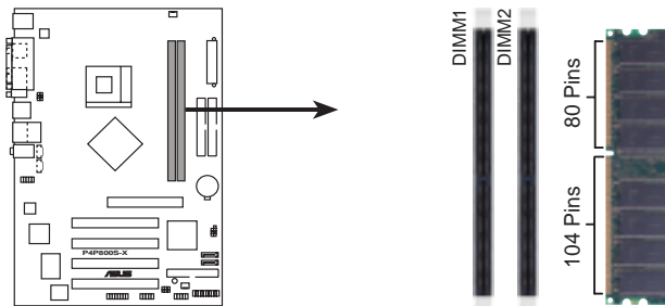
P4P800S-X 184-Pin DDR DIMM Sockets
