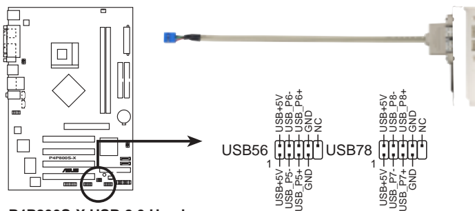
P4P800S-X USB 2.0 Headers
