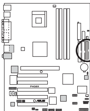
P4G8X Floppy Disk Drive Connector
