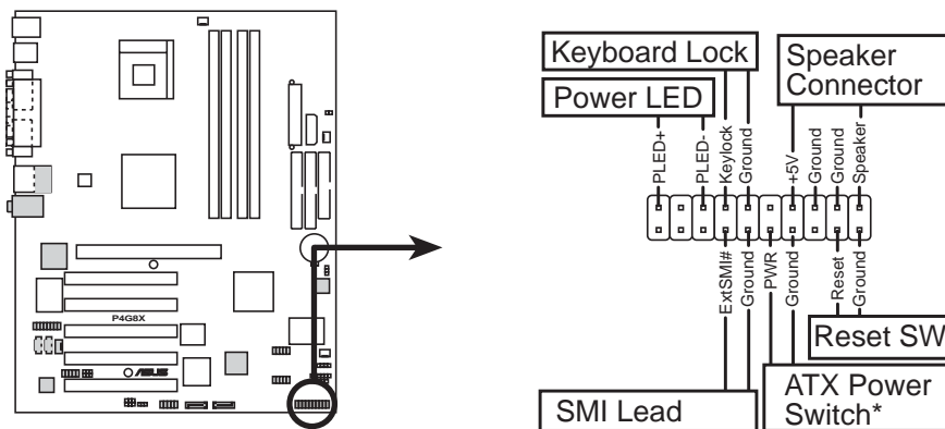
P4G8X System Panel Connectors
