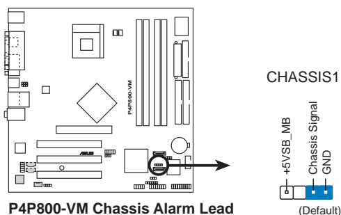
P4P800-VM Chassis Alarm Lead
