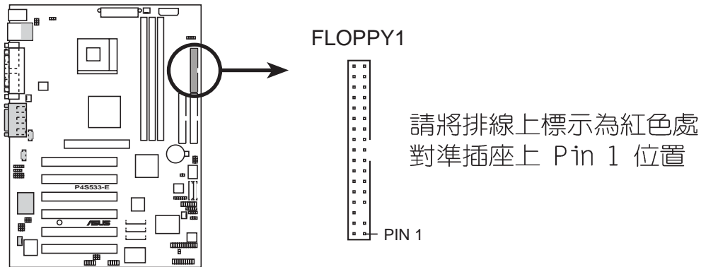
P4S533-E Floppy Disk Drive Connector
