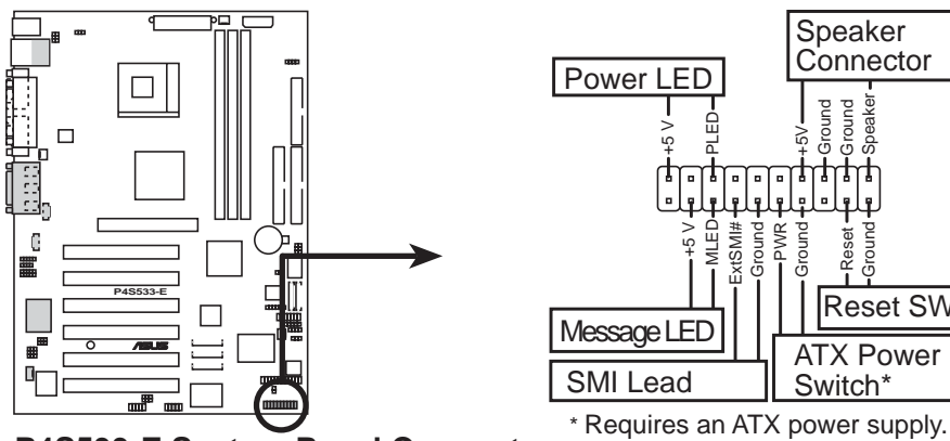
P4S533-E System Panel Connectors
