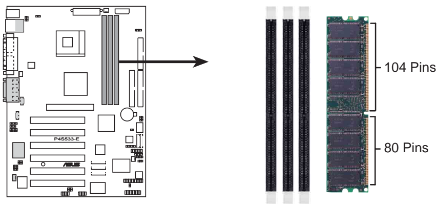
P4S533-E 184-Pin DDR DIMM Sockets
