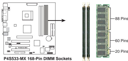
P4S533-MX 168-Pin DIMM Sockets
