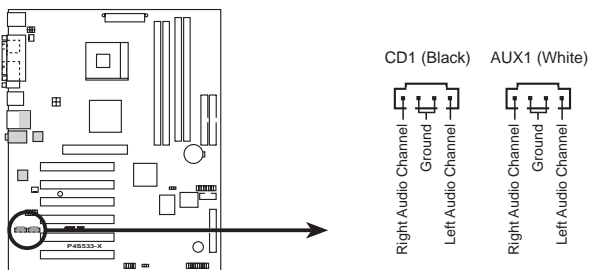
P4S533-X Internal Audio Connectors
