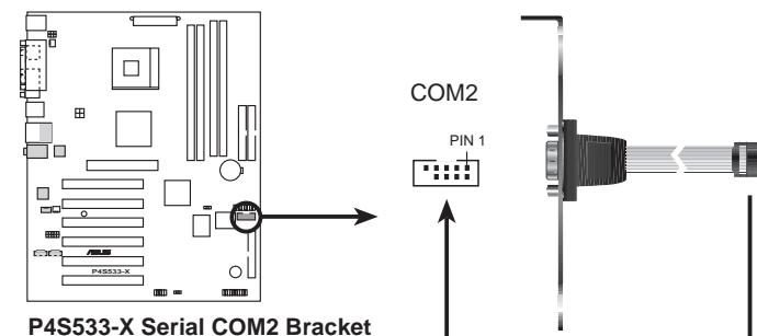
P4S533-X Serial COM2 Bracket
