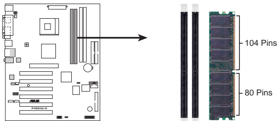
P4S533-X 184-Pin DDR DIMM Sockets
