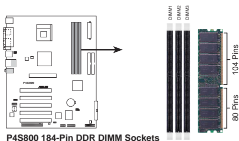
P4S800 184-Pin DDR DIMM Sockets
