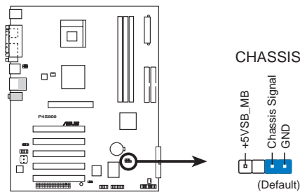
P4S800 Chassis Alarm Lead
