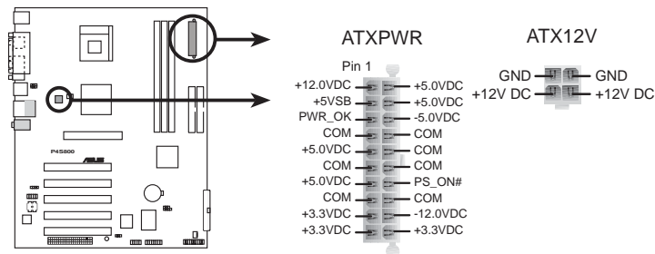
P4S800 ATX Power Connector
