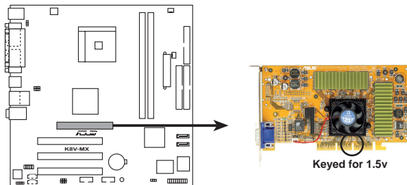
K8V-MX Accelerated Graphics Port (AGP)
