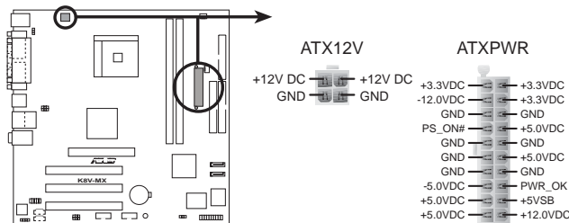
K8V-MX ATX power connectors
