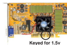
K8V SE Deluxe Accelerated Graphics Port (AGP)
