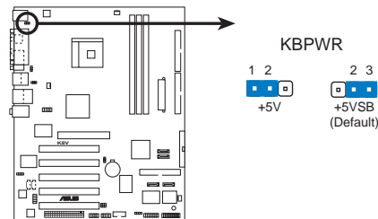
K8V SE Deluxe Keyboard Power Setting
