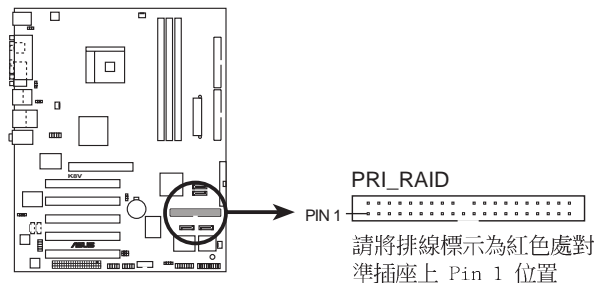
K8V SE Deluxe RAID Connectors
