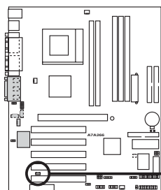
A7A266 Wake-On-LAN Connector
