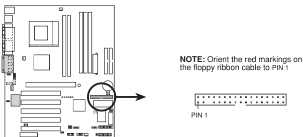
A7A266 Floppy Disk Drive Connector
