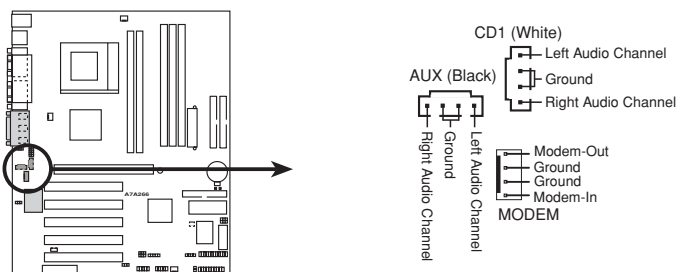
A7A266 Internal Audio Connectors
