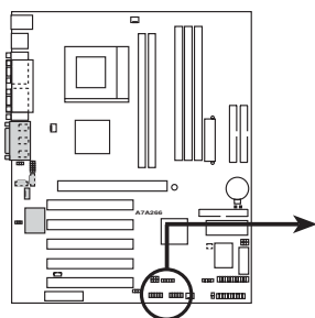
A7A266 Front Panel USB Headers
