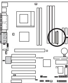
A7A266 ATX Power Connector
