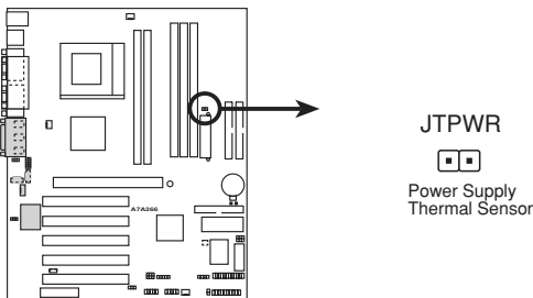
A7A266 Thermal Sensor Connector
