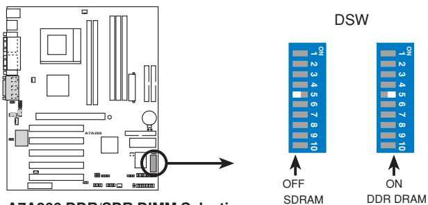
A7A266 DDR/SDR DIMM Selection
