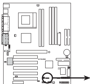
A7A266 SMBus Connector
