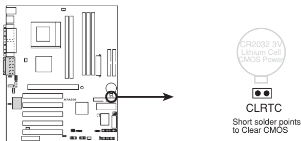
A7A266 Clear RTC RAM
