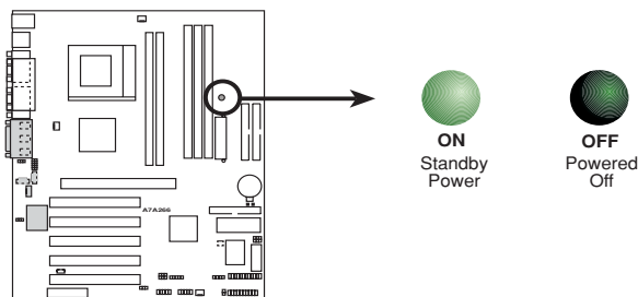
A7A266 Onboard LED
