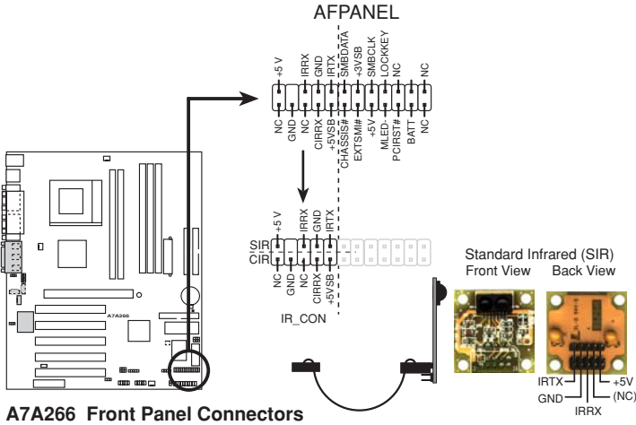
A7A266 Front Panel Connectors
