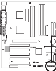
A7A266 System Panel Connectors
