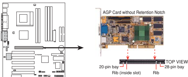
A7A266 Accelerated Graphics Port (AGP PRO)
