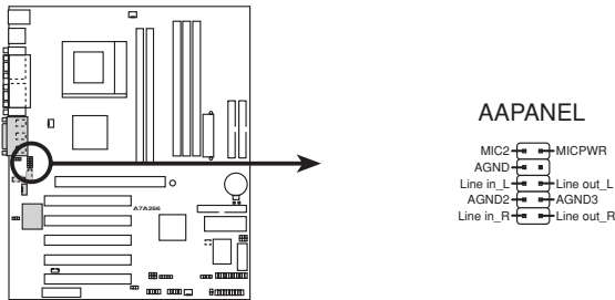
A7A266 Audio Panel Connector
