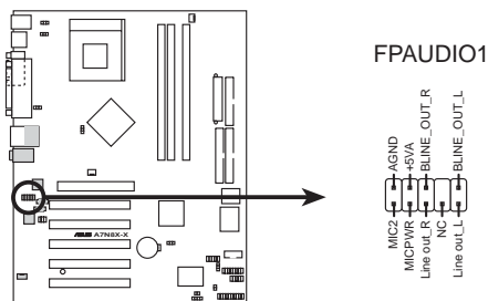
AT7N8X-X Front Panel Audio Connector
