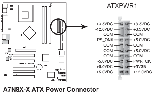
AT7N8X-X ATX Power Connector
