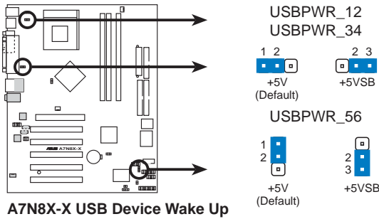
A7N8X-X USB Device Wake Up
