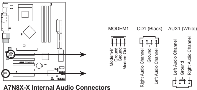
A7N8X-X Internal Audio Connectors
