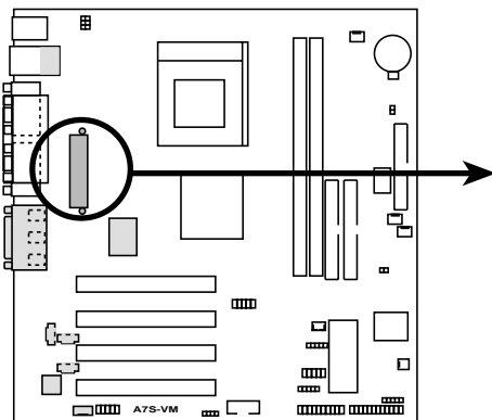
A7S-VM ATX Power Connector
