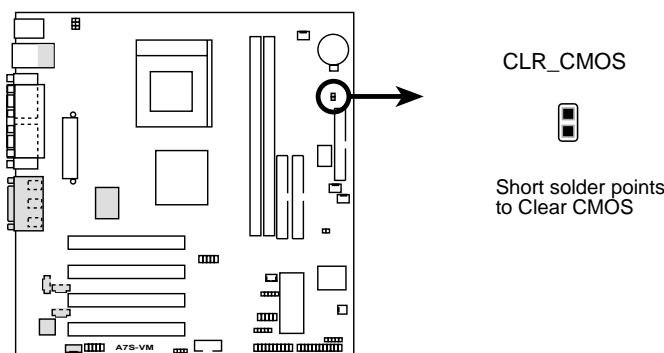
A7S-VM Clear RTC RAM
