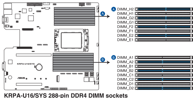
KRPA-U16/SYS 288-pin DDR4 DIMM sockets
