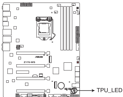
Z170-WS TPU LED
