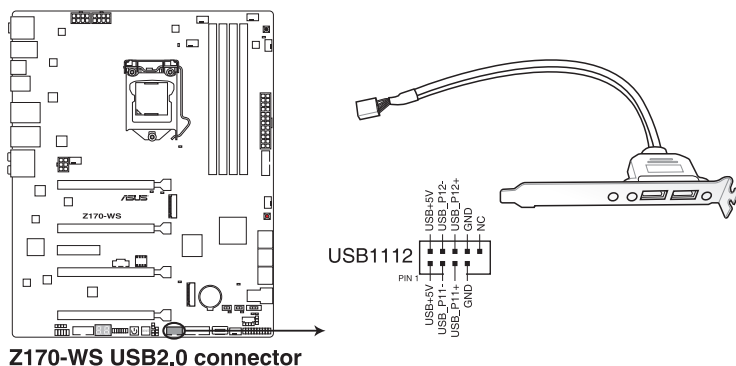
Z170-WS USB2.0 connector
