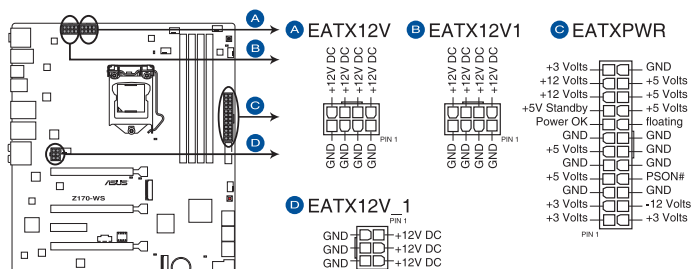
Z170-WS ATX power connectors
