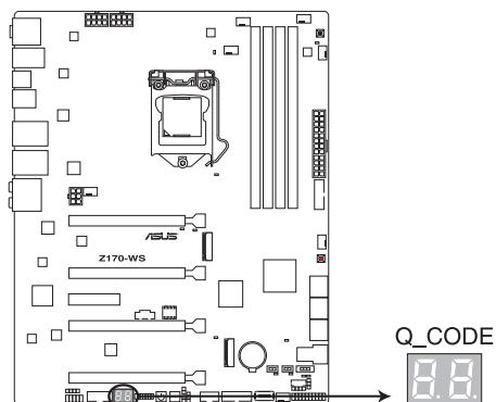
Z170-WS Q-Code LED
