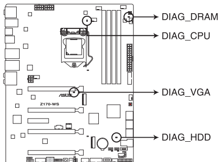
Z170-WS Diagnosis LED
