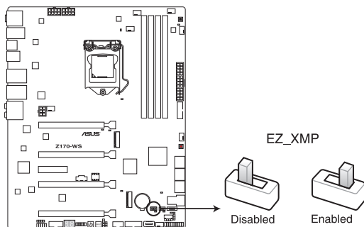
Z170-WS EZ_XMP switch
