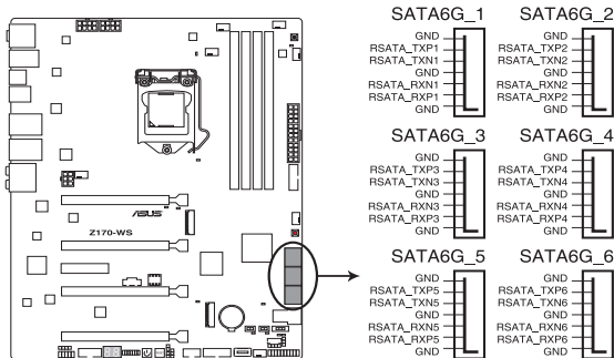
Z170-WS Intel® SATA 6 Gb/s connectors
