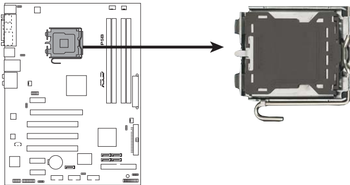
P5B CPU-Sockel 775
