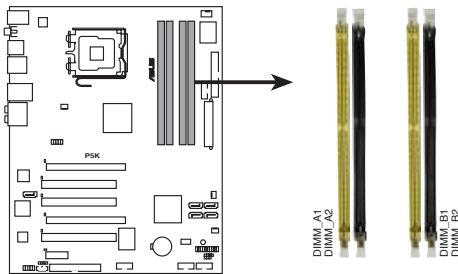
P5K 240-pin DDR2 DIMM Slots
