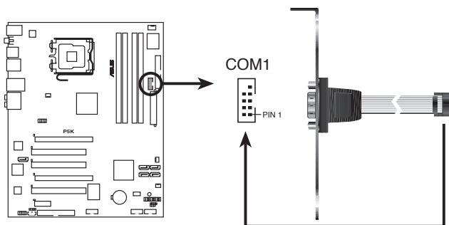
P5K COM port connector
