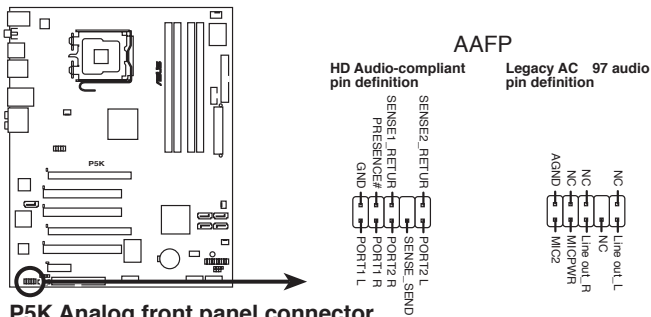
P5K Analog front panel connector
