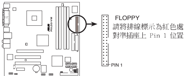
P5LD2-VM Floppy disk drive connector
