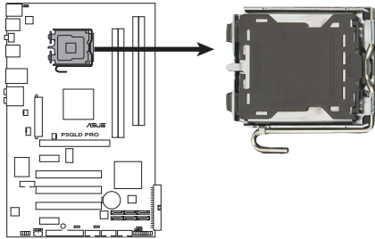
P5QLD PRO CPU Socket 775
