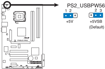
P5QLD PRO Keyboard Power Setting
