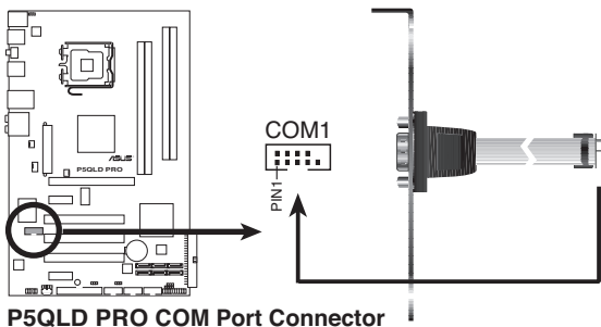
P5QLD PRO COM Port Connector
