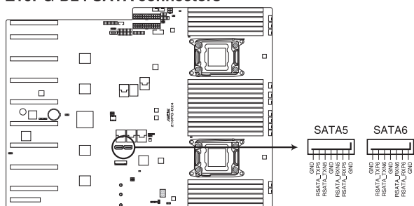
Z10PG-D24 SATA connectors
