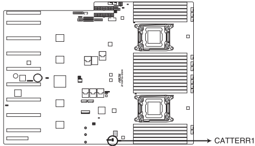
Z10PG-D24 CATTERR LED
