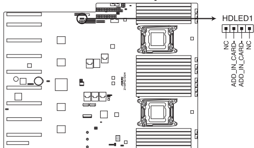
Z10PG-D24 Hard disk activity LED connector
