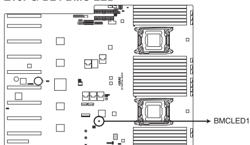
Z10PG-D24 BMC LED
