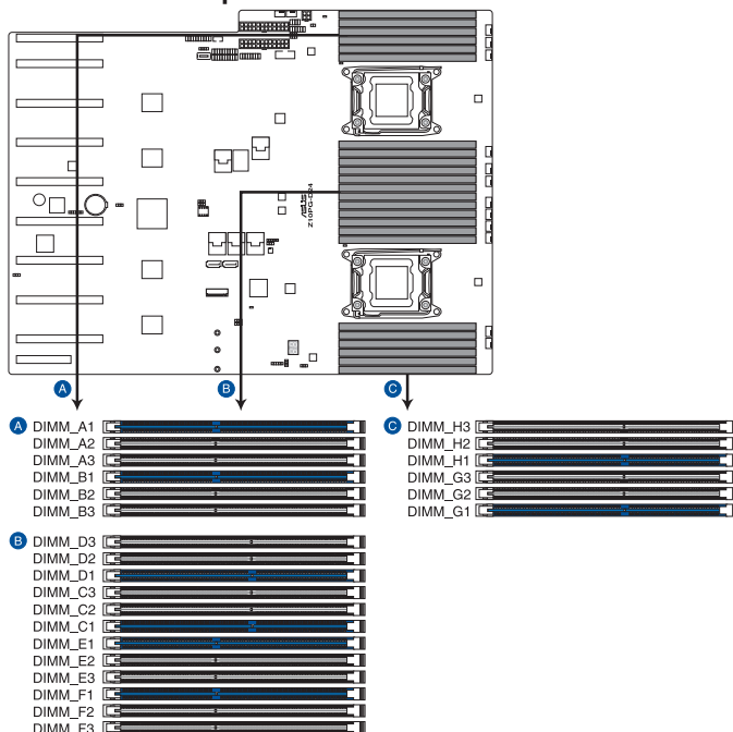
Z10PG-D24 288-pin DDR4 DIMM sockets
