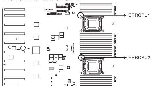
Z10PG-D24 ERR CPU LED
