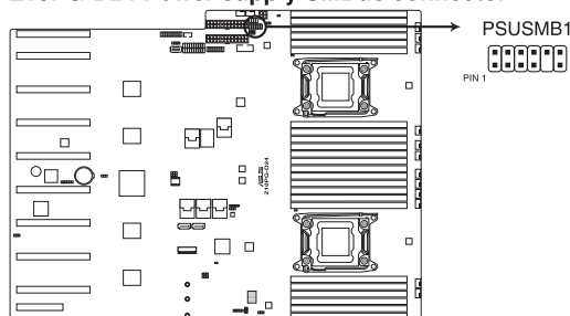
Z10PG-D24 Power supply SMBus connector
