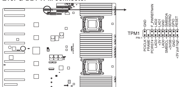
Z10PG-D24 TPM connector
