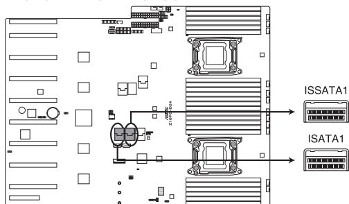
Z10PG-D24 ISATA & ISSATA connectors
