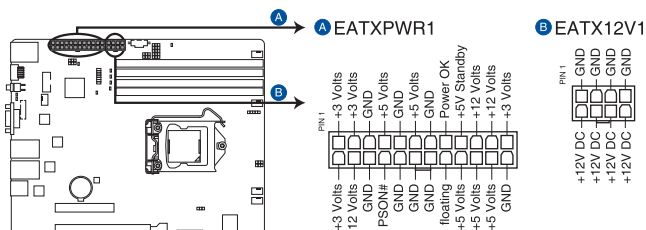
P11C-M/4L ATX power connectors
